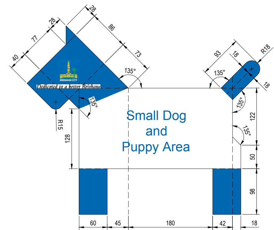
DOG OFF-LEASH SIGN - 2 PANEL B DETAIL SCALE: 1:5
